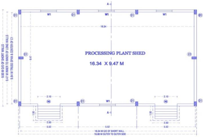
PROCESSING PLANT SHED PLAN
